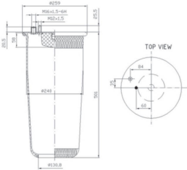
MAN 81.43601.0153
