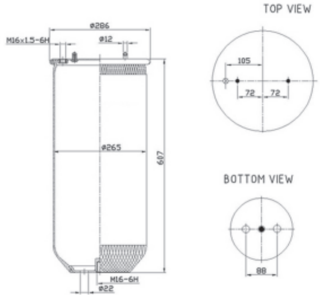
SCANIA 1379393
