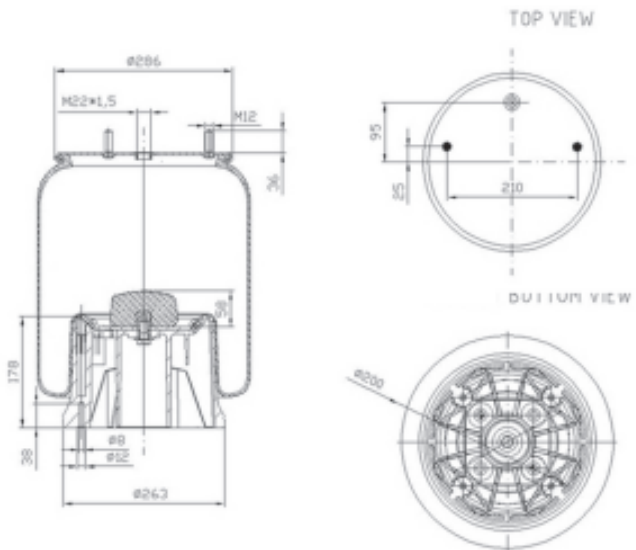
SAF 3.229.0028.00
